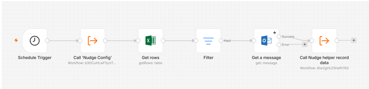
Figure 7. “Check Unprompted” Main workflow
