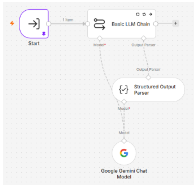
Figure 9. “Followup prompt” Helper workflow
